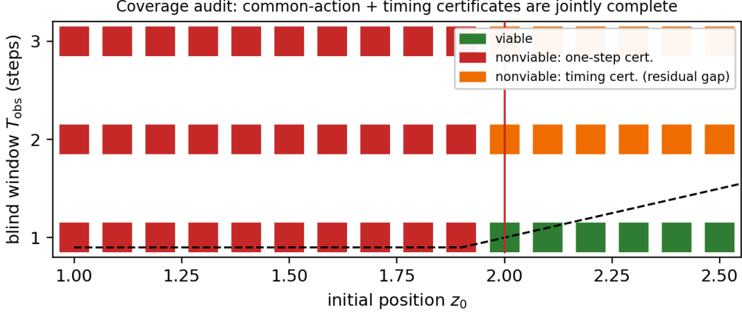
Figure 3: Whole-window hold-class coverage of Table 2: green = viable; red = nonviable under either class, certified by the common-action certificate; orange = nonviable only in the audited hold class , certified there by the timing bound. With per-step alternating actions, the orange cells are viable. The dashed curve is the hold-class boundary z_0 = 1 + T_{\text{obs}} , not an unrestricted boundary; the solid vertical line marks the one-step boundary z_0 = 2 .
